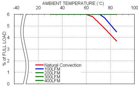
DOS06-05T, Vout=3.3V Derating Curve
