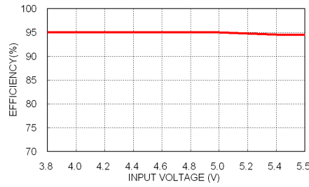
DOS06-05T, Vout=3.3V Efficiency vs. Input Voltage
